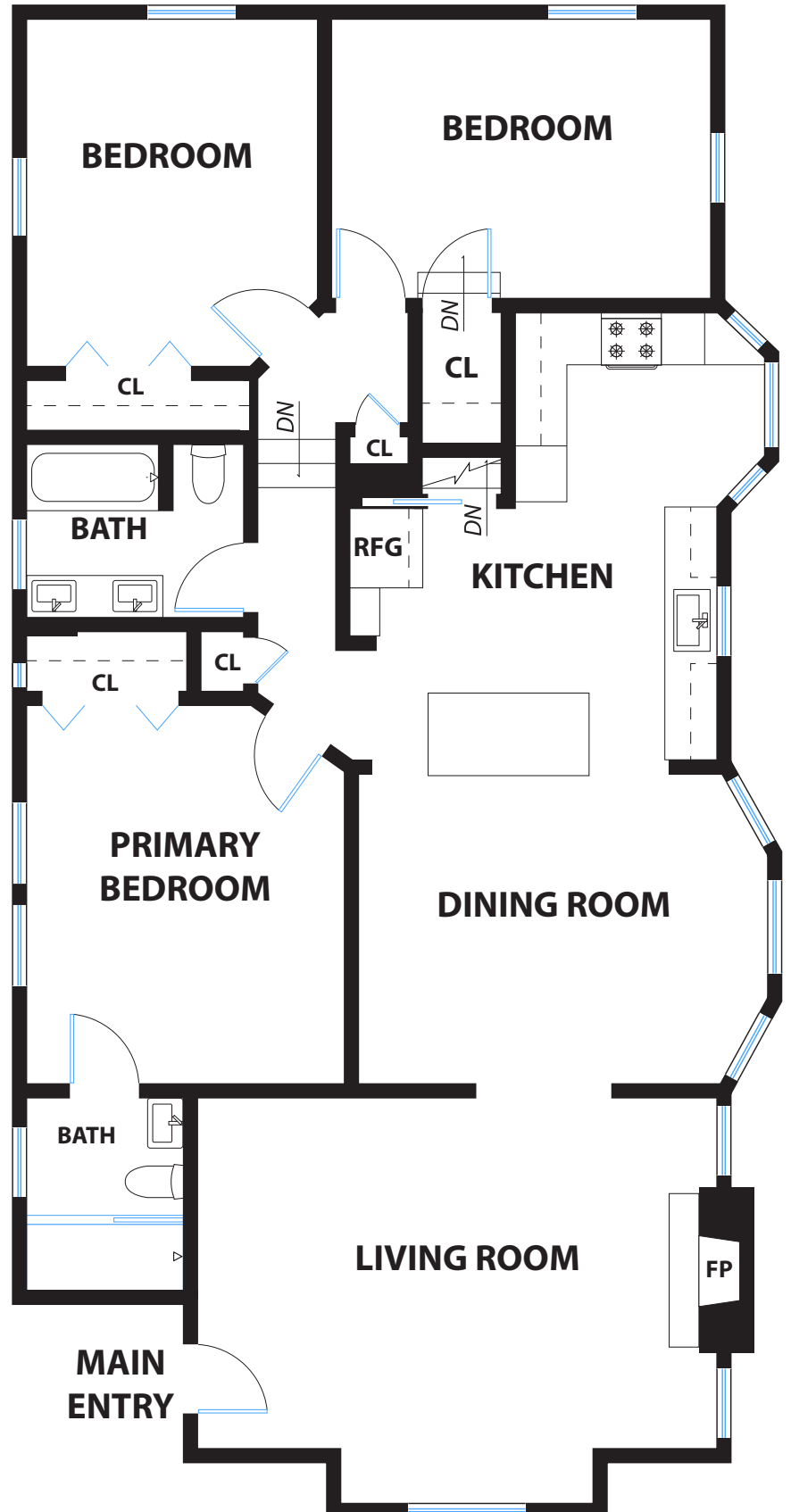
SECOND FLOOR
